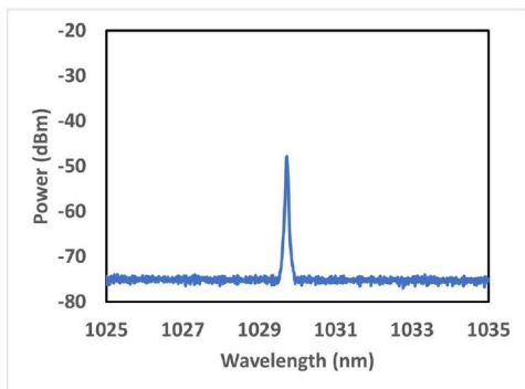
Fig. 3. OEPLS-PS-100-NL Seed module spectrum
