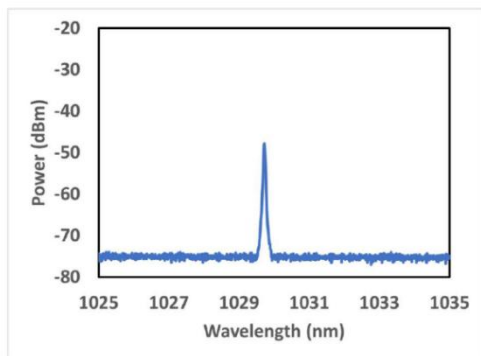
Fig. 3. OEPLS-PS-100-NL Seed module spectrum
