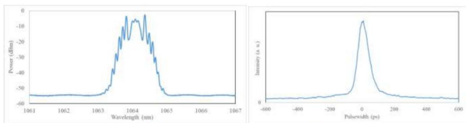
OEPLS-PS-100 spectrum and pulse shape at 1060 nm.
