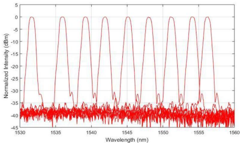
Fig.1. FBG reflection spectra over the tuning range.
