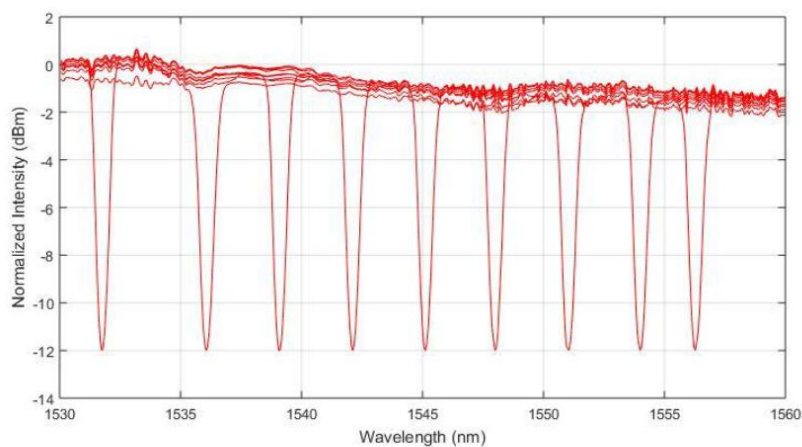
Fig.2. FBG transmission spectra over the tuning range.
