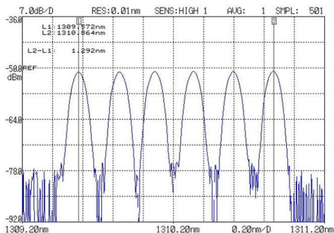
Fig.2. FBG reflection spectra over the tuning range.
