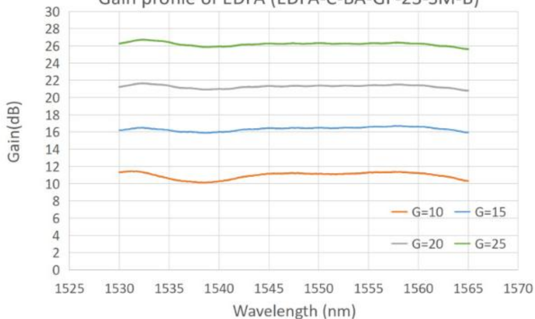
Gain profile of EDFA (EDFA-C-BA-GF-23-SM-B)
