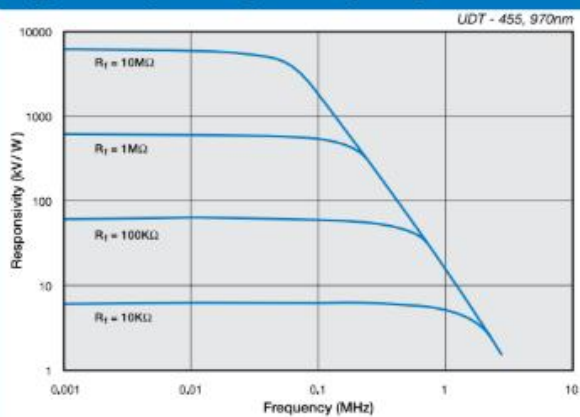
Typical Responsivity vs. Frequency
