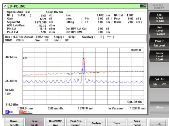
1278 nm (Pin = 0 dBm, I = 200mA)
