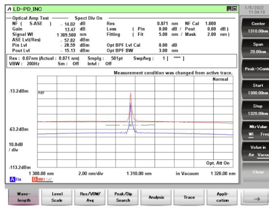
1310 nm (Pin = 0 dBm, I = 200mA)
