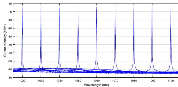
Output spectrum of OETLS-300 at 1060 nm
