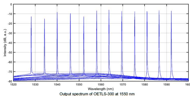
Output spectrum of OETLS-300 at 1550 nm
