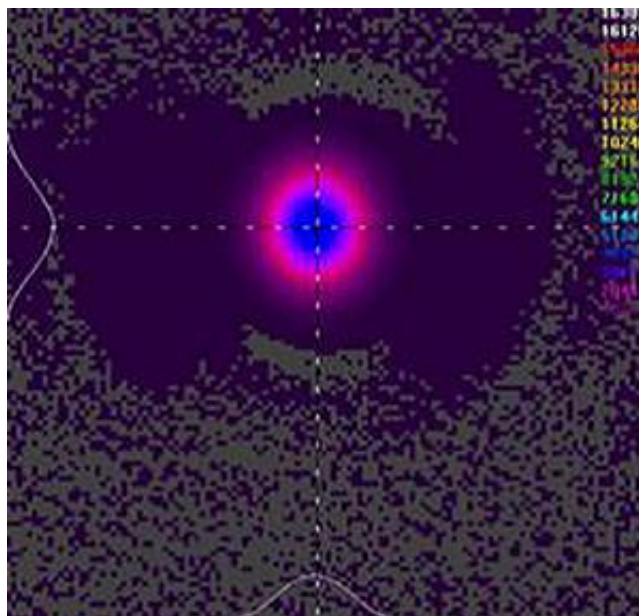
3-D Beam Profile at 1778 mm (70.0 in)
