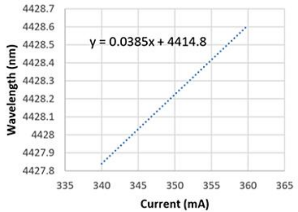
Wavelength Tuning at 25C
