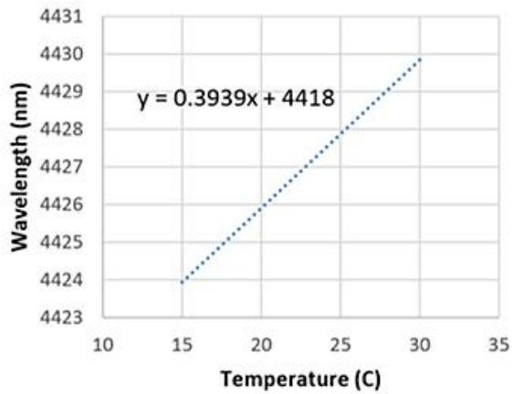
Wavelength Tuning at 340mA
